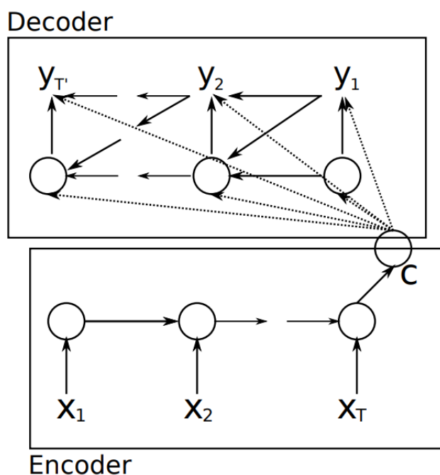
Figure 28.2: Depiction of the Encoder-Decoder architecture. Taken from Learning Phrase Representations using RNN Encoder-Decoder for Statistical Machine Translation .
